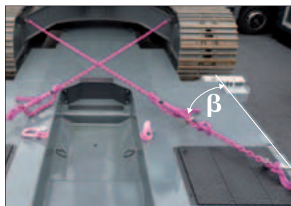
Horizontal angle \beta
